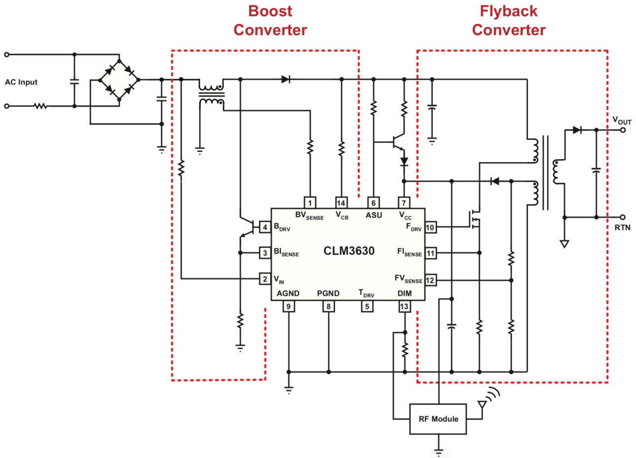
Figure 3.3 : CLM3630 Wireless Dimming Simplified Schematic
