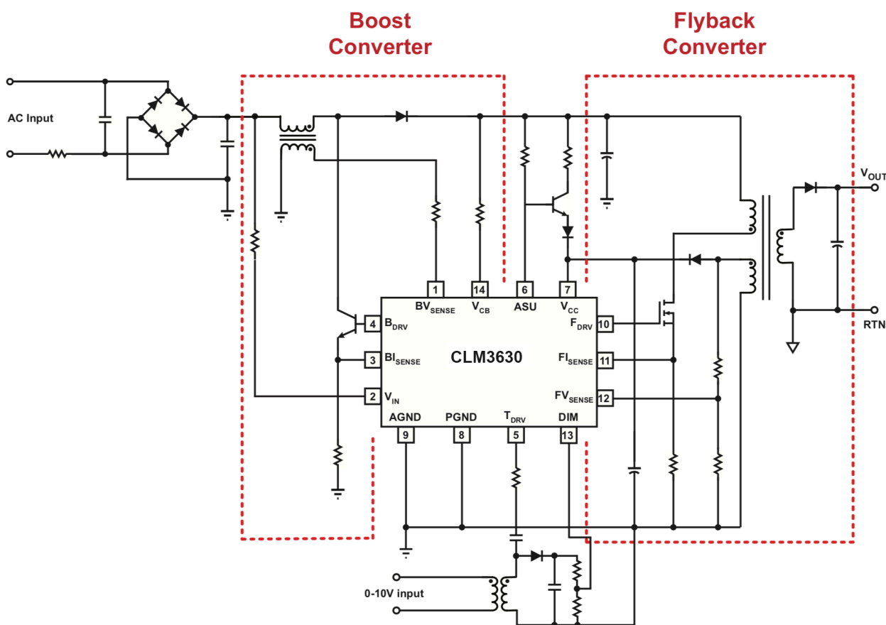
3.2 : CLM3630 0-10V Dimming Simplified Schematic
