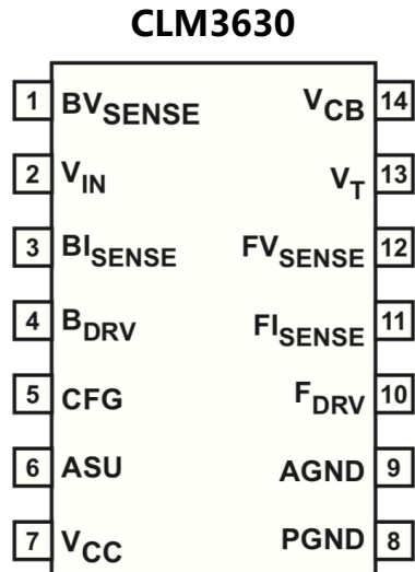
Figure 4.1 : 14-Lead SOIC Package
