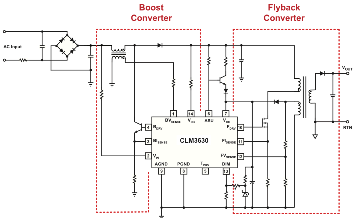
Figure 3.1 : CLM3630 Dimming Simplified Schematic
