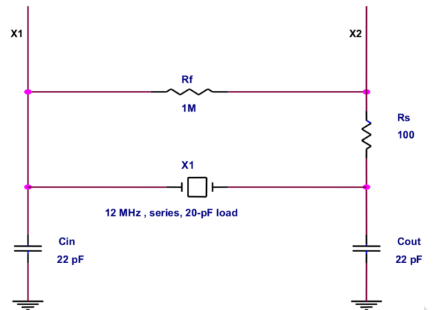
Figure 3. Optional 12 MHz Crystal Circuit Typical Crystal Requirements
