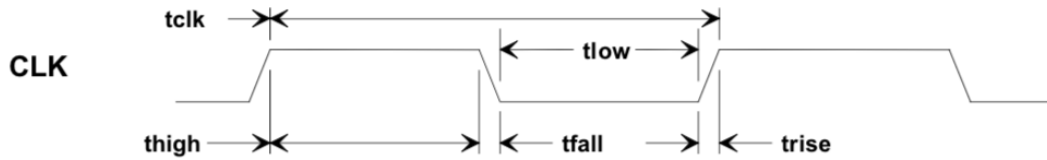
Clock Timing
