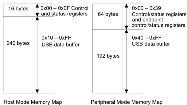
Figure 1. Memory Map
