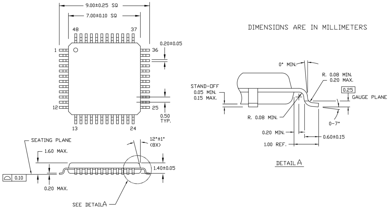
Figure 7. 48-pin TQFP (7 × 7 × 1.4 mm) Package Outline, 51-85135
