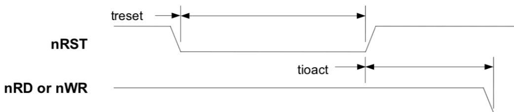
Reset Timing
