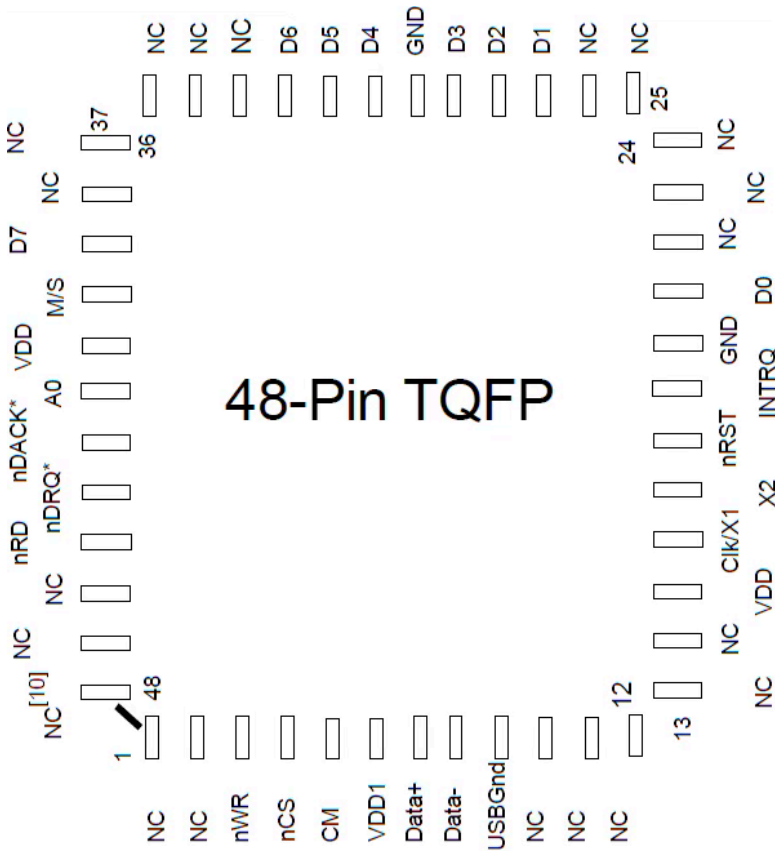
Figure 4. 48-pin TQFP AXC USB Host/Slave Controller Pin Layout
