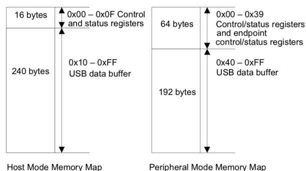
Figure 1. Memory Map
