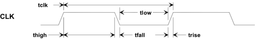
Clock Timing
