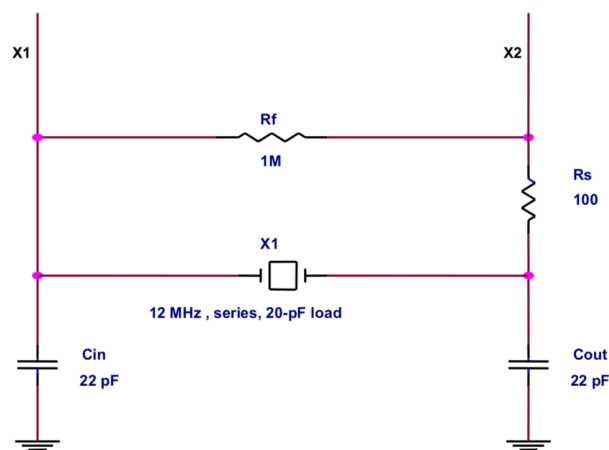
Figure 3. Optional 12 MHz Crystal Circuit Typical Crystal Requirements
