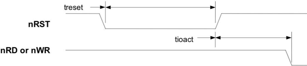
Reset Timing
