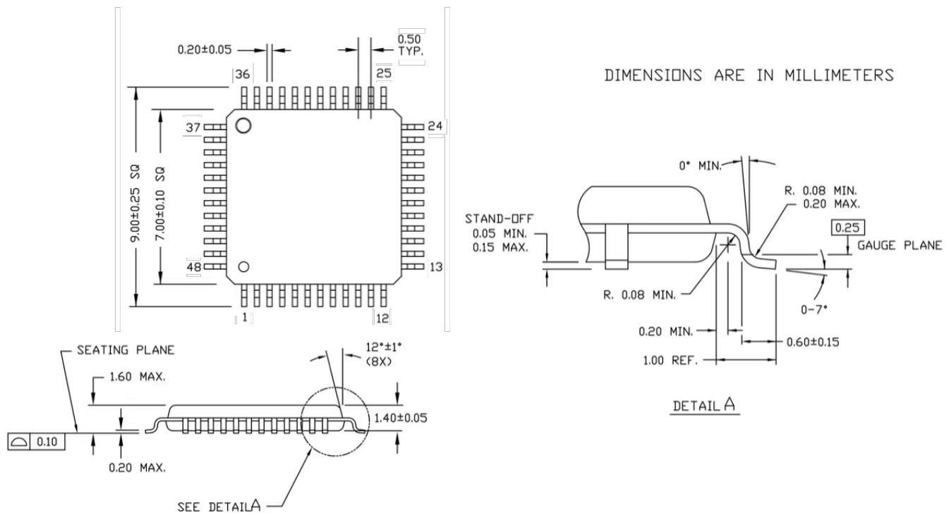
Figure 7. 48-pin TQFP (7 × 7 × 1.4 mm) Package Outline, 51-85135
